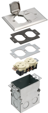
Single Gang
